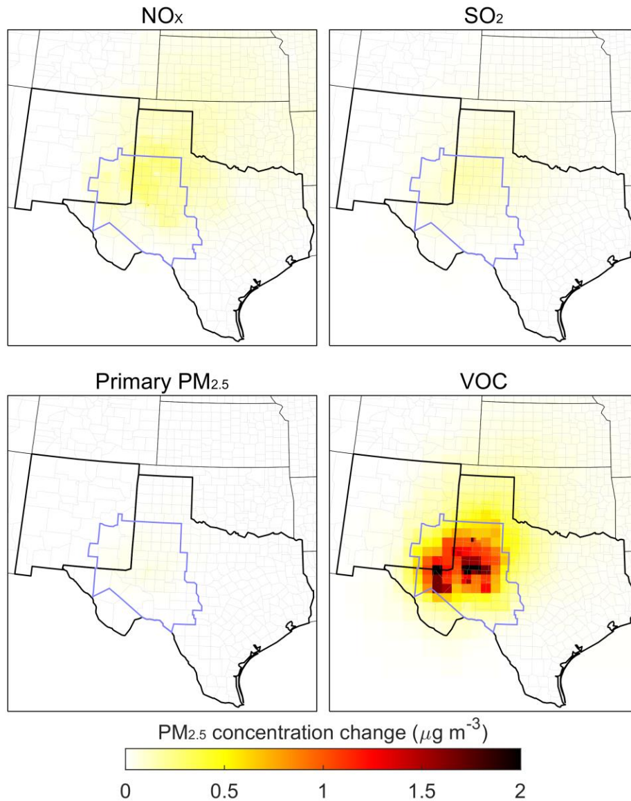
Figure 10: Modeled PM 2.5 concentration changes ( \mu\text{g}/\text{m}^3 ) in 2017 attributable to Permian Basin oil and gas emissions, by precursor pollutant type. 1×1 km to 48×48 km gridded data shown (varied based on population density). Permian Basin region outlined in blue. Sources: Goodkind et al. (2019) and authors' modeling results.
